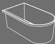
Febe Vasca freestanding Bath tub freestanding cm 140 x 80 x 57 h
