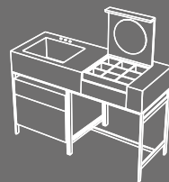
Narciso vanity Con cassettera With drawer unit cm 130 x 50 x 83 h
