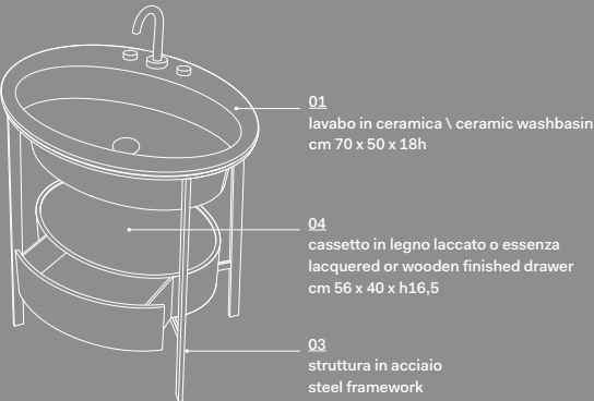
Catino Ovale 70 monoforo predisposto 3 fori, con cassetto with 1 hole prepared 3 holes, with drawer - cm 70 x 50 x h83
