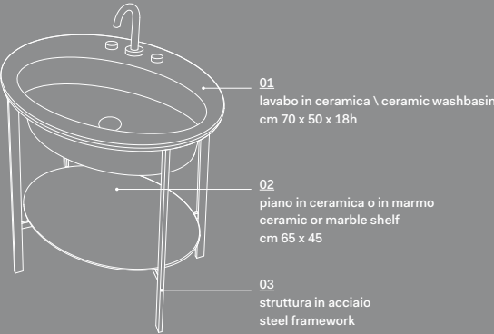
Catino Ovale 70 monoforo predisposto 3 fori, con piano \ with 1 hole prepared 3 holes, with shelf - cm 70 x 50 x h83
