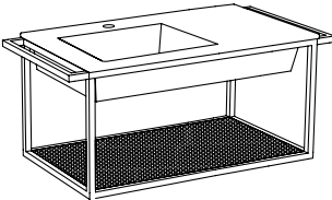
LAVABO ERA 60 BACINO SINISTRO Era 60 washbasin with basin on the left cm 60 x 46 x 42 h
