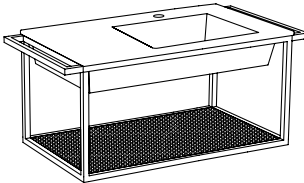
LAVABO ERA 60 BACINO DESTRO Era 60 washbasin with basin on the right cm 60 x 46 x 42 h
