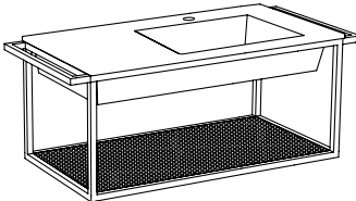
LAVABO ERA 80 BACINO DESTRO Era 80 washbasin with basin on the right cm 80 x 46 x 42 h
