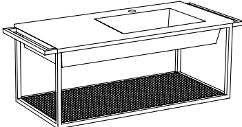
LAVABO ERA 100 BACINO DESTRO Era 100 washbasin with basin on the right cm 100 x 46 x 42 h
